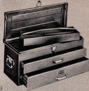
Heavy-duty steel chest is 25x10x11 inches over all; has two deep drawers and 19x7½-inch lift-out "tote" tray.
